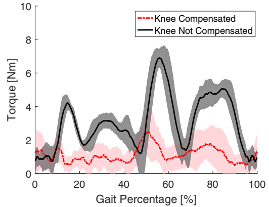
(a) Knee Backdrive Torque
