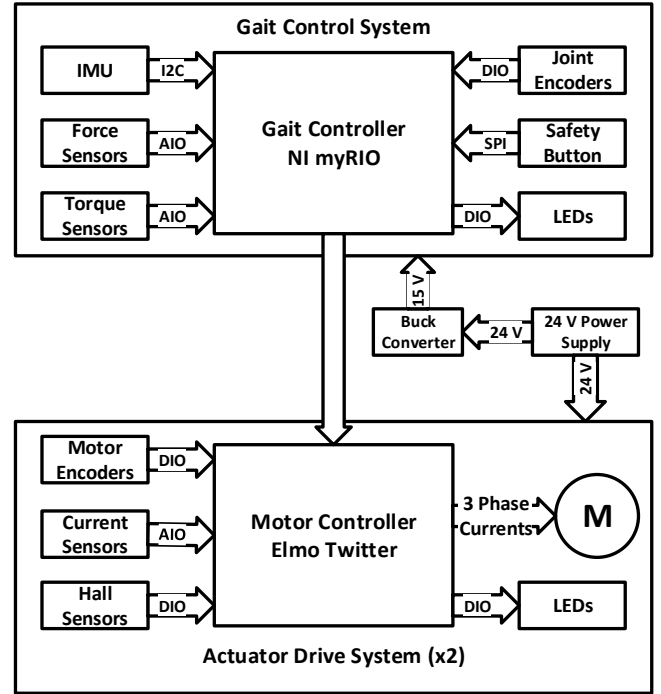
Fig. 5. Block Diagram of Electrical System: The gait control system receives feedback related to the user's gait and sends torque commands. The two actuator drive systems control and drive the knee and ankle actuators. A buck DC-DC converter provides power to the gait control system.
